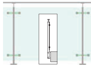
218 Glass adapters - spider MOD 4752
